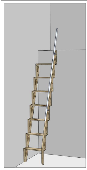
Ladder above with OPTIONAL short, fixed handrail
